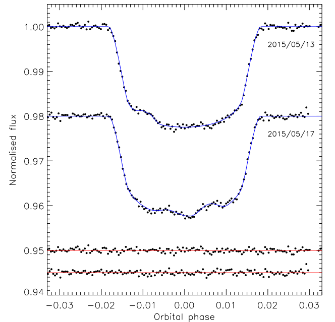
Figure 8. Best fits from PRISM+GEMC for the third (upper) and fourth (lower) transits we observed with DFOSC.
