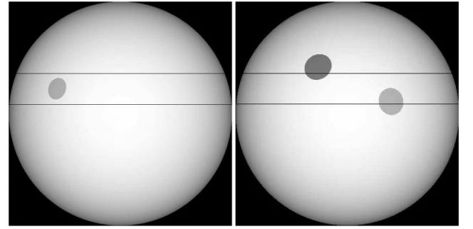
Figure 7. Visualizations of the surface of WASP-41 A at the times of the third (left) and fourth (right) transits we observed with DFOSC, produced by PRISM. The boundaries of the path of the planet are shown with black lines and the spots are shown with their measured locations, sizes and contrasts.
