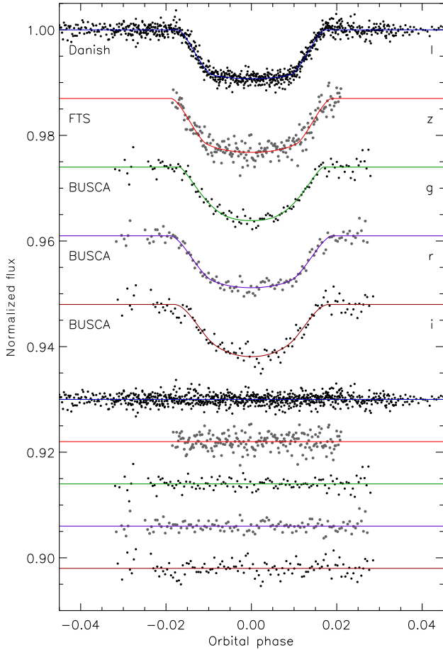
Figure 7. The phased light curves of WASP-26 analysed in this work, compared to the \text{JKTEBOP} best fits. The residuals of the fits are plotted at the base of the figure, offset from unity. Labels give the source and passband for each data set. The polynomial baseline functions have been removed from the data before plotting.
