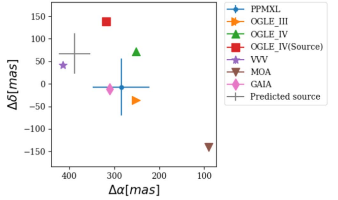
Figure 5. Location of the target from the catalogs listed in the Table 4, centered at (R.A. = 271.6826°, Decl. = −32.9076°) (J2000). North is up and east is left. Some uncertainties have been hidden for clarity. The source position measured from OGLE-IV is located at \Delta(E, N) = (78, 78) mas (red square) from the OGLE-IV position. The gray cross indicates the prediction of the source, applying the offset to the Gaia position and assuming \sigma(N, E) = (45, 35) mas uncertainties.
